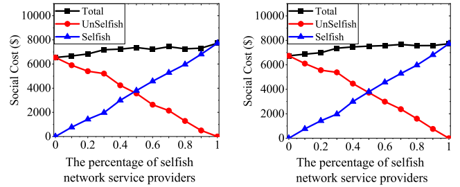
(a) The impact of 1 - \xi on the performance of the LECF
