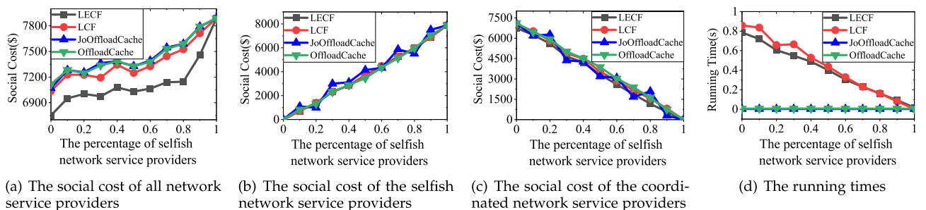
Fig. 4. The impact of (1 - \xi) on the algorithm performance with size 200.
