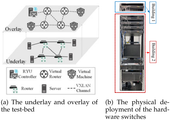
Fig. 5. A test-bed with both hardware switches and virtual resources.
