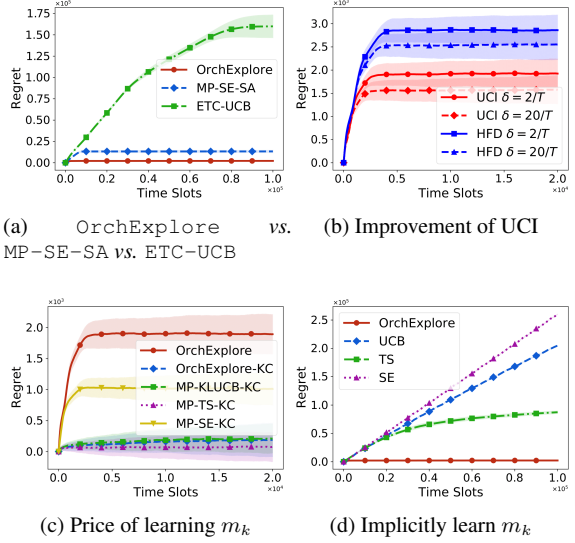
Figure 1. Evaluation under Bernoulli Rewards
