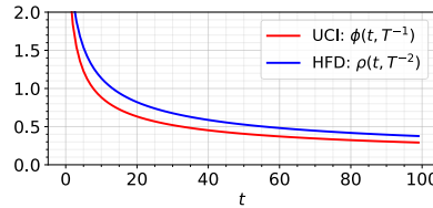
Figure 5. Our UCI's \phi(t, T^{-1}) v.s. the one based on Hoeffding's inequality (HFD)'s \rho(t, T^{-2}) ( T = 10^6 ).
