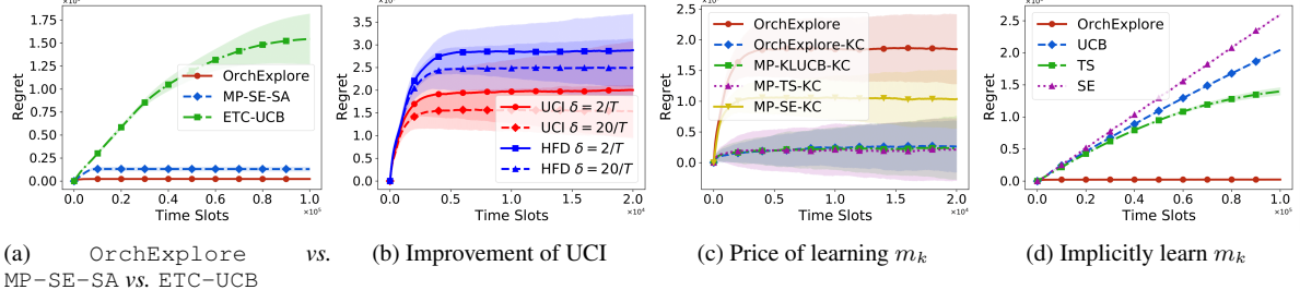
Figure 4. Evaluation under Gaussian Distributions with 1/2 Variance
