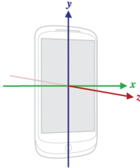
Fig 4.2.3 Device orientation
