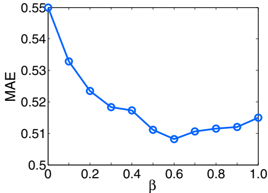
Fig. 5. Impact of \beta on HMF
