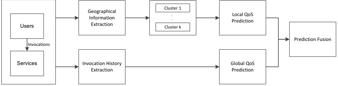
Fig. 2. Framework of Hierarchical Web Service Recommendation System
