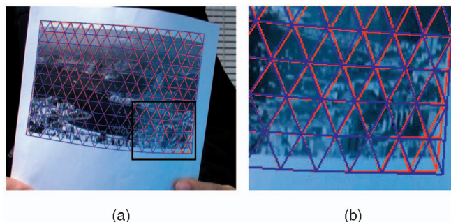
Fig. 16. Comparison of the deformable Lucas-Kanade (DLK) method (blue) and the fusion approach (red) on the paper video. Results are shown at frame 251. (a) Frame 251. (b) Zoomed region.
