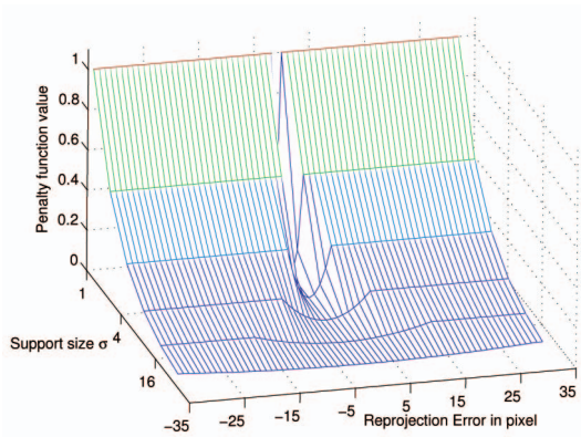
Fig. 5. The robust estimator that assesses a fixed penalty to residuals larger than a threshold \sigma .
