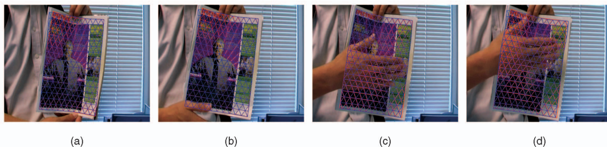
Fig. 15. Comparison of the deformable Lucas-Kanade (DLK) method (blue) and the fusion approach (red) on the magazine video. The magazine cover is occluded by hand in (c) and (d). (a) Frame 80. (b) Frame 229. (c) Frame 249. (d) Frame 271.
