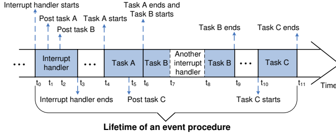
Figure 1. A sample event procedure instance.
