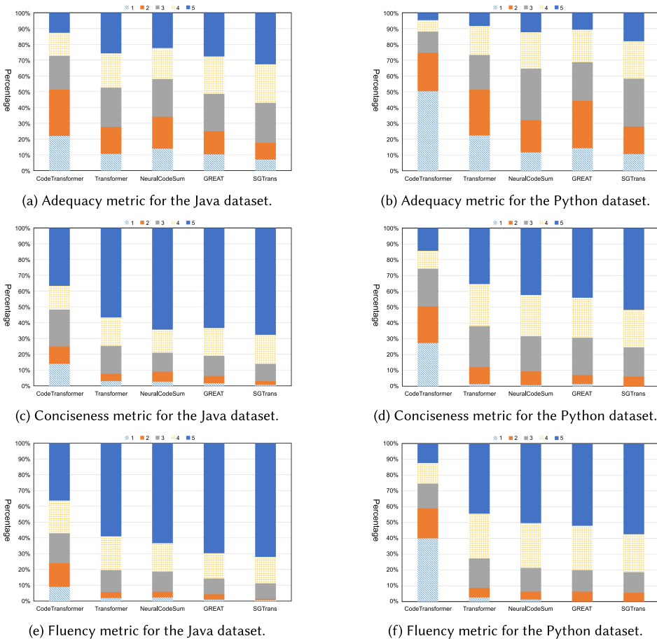
Fig. 7. Distribution of the rating scores in human evaluation on the two datasets. The “Transformer” on the horizontal axis denotes the “vanilla Transformer” approach.
