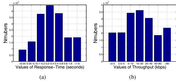
Figure 3. Value Distributions
