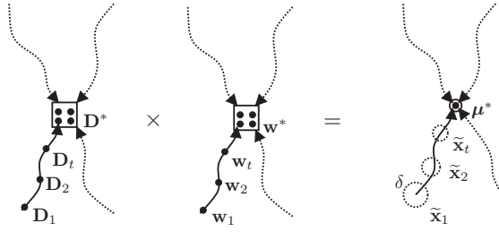
Fig. 1. The schematic diagram of how the algorithm of online dictionary learning via moment information works intuitively.
