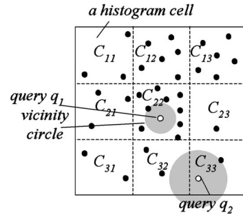
Fig. 6. Histogram example.
