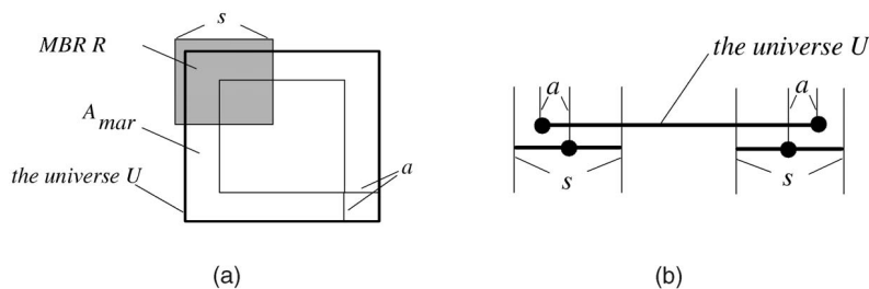
Fig. 21. The integral area. (a) 2D case. (b) 1D version of the problem.
