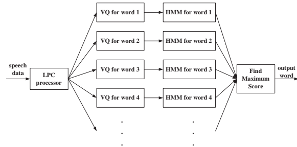
Figure 1: Isolated word recognition system
