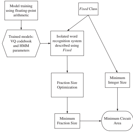
Figure 5: Design flow
