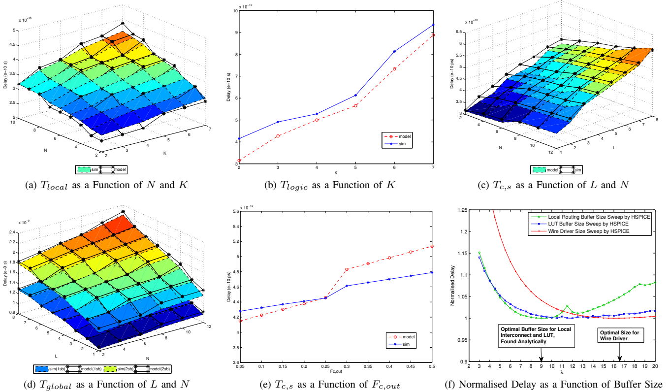
Fig. 11. Delay Model Comparison with HSPICE
