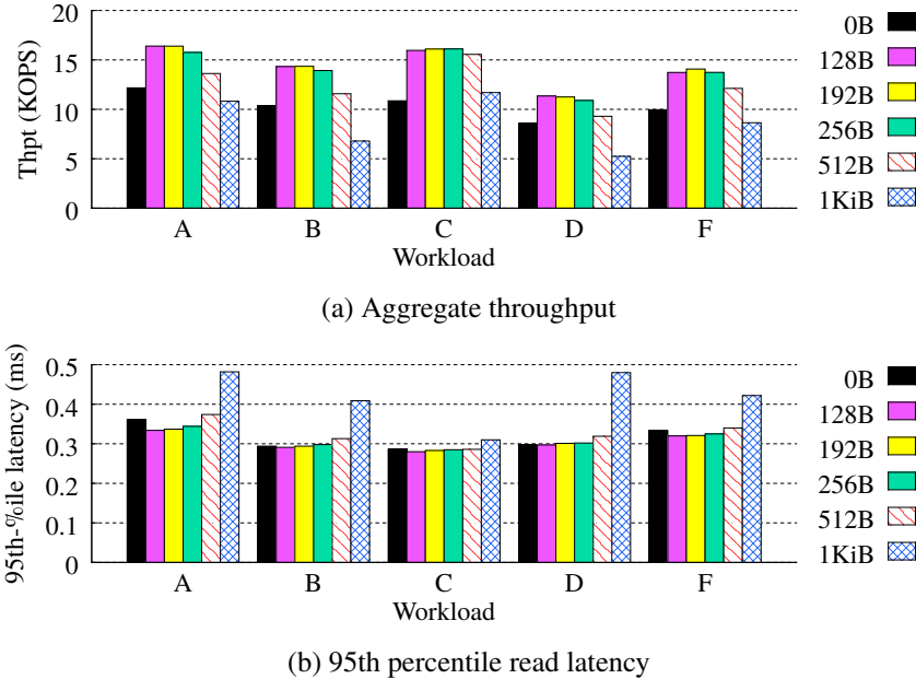
Figure 16: Experiment 12: Threshold selection of selective KV separation under YCSB core workloads.
