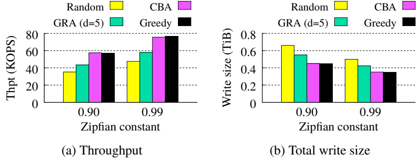
Figure 14: Experiment 9: Impact of GC approaches.
