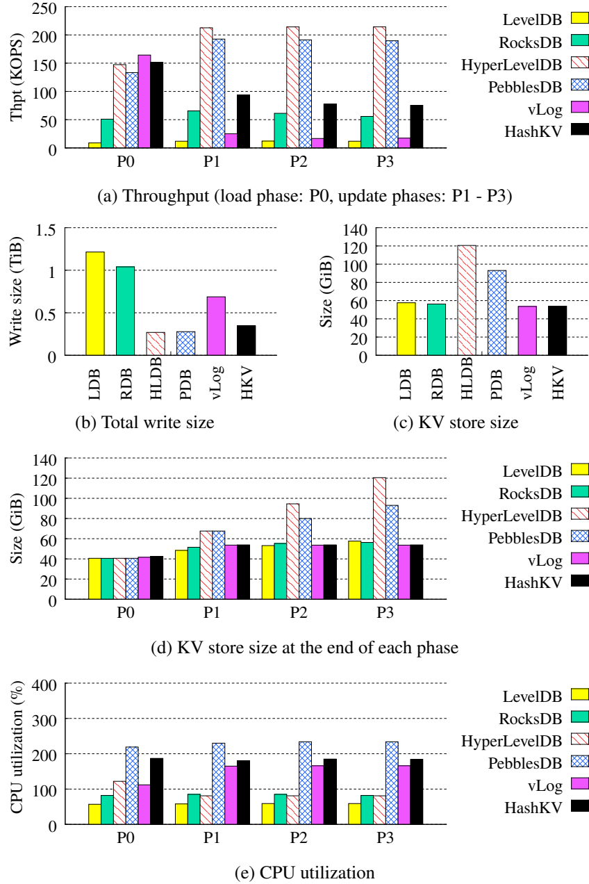
Figure 6: Experiment 1: Performance comparison of KV stores under update-intensive workloads.
