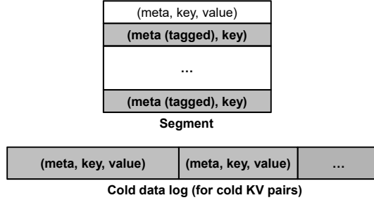
Figure 4: Tagging in HashKV. Note that the locations of the cold KV pairs in the cold data log are stored in the LSM-tree.
