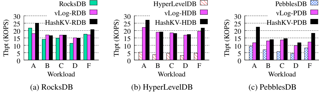
Figure 17: Experiment 13: Deployment of KV separation on different KV stores under YCSB core workloads.
