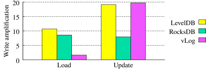
Figure 2: Write amplifications of LevelDB, RocksDB, and vLog in the load and update phases.
