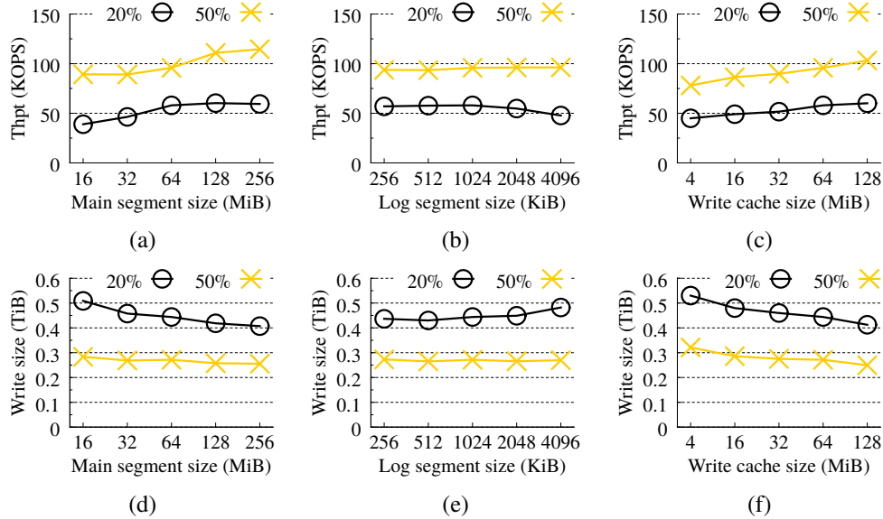
Figure 20: Experiment 15: Throughput and total write size of HashKV versus the main segment size ((a) and (d)), the log segment size ((b) and (e)), and the write cache size ((c) and (f)).
