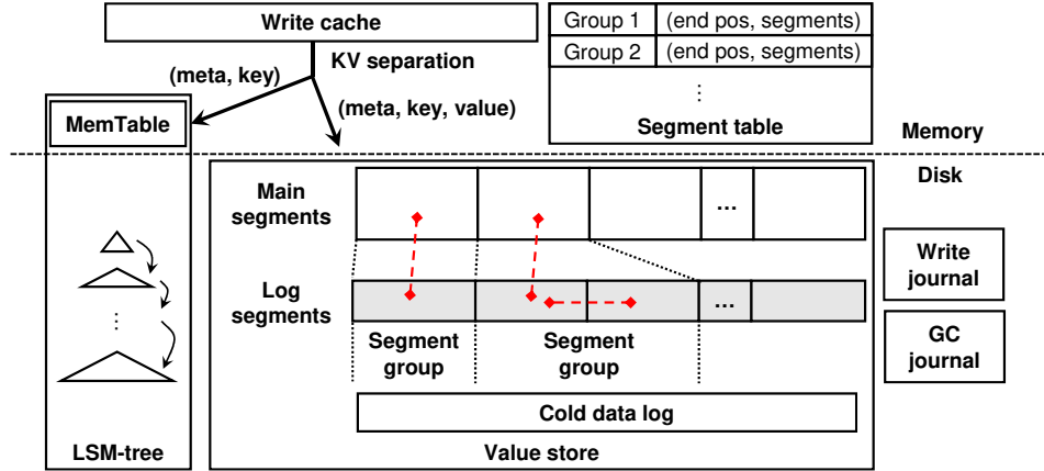
Figure 3: HashKV architecture. Each segment group consists of one main segment and a variable number (zero or more) of log segments; the log segments (in shaded color) are provisioned in reserved space. For example, the segments that are linked together belong to the same segment group.
