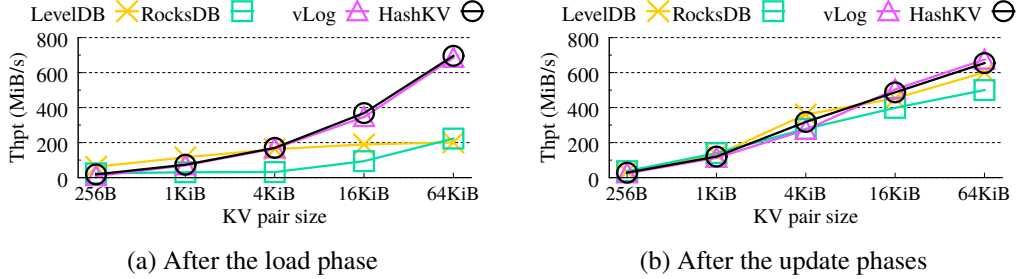
Figure 10: Experiment 5: Range scan performance versus the KV pair size.
