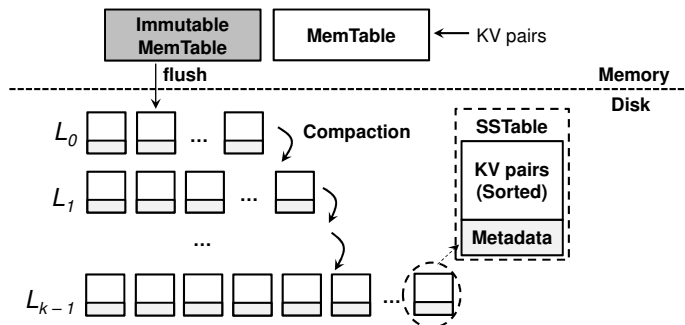
Figure 1: Data organization in LevelDB.
