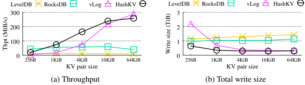
Figure 9: Experiment 4: Update performance versus the KV pair size.
