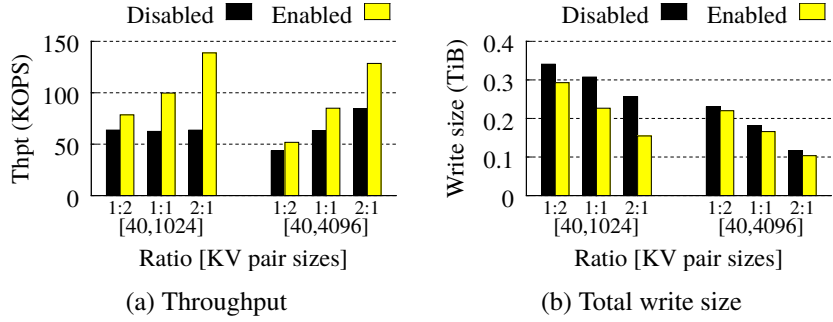
Figure 12: Experiment 7: Selective KV separation.
