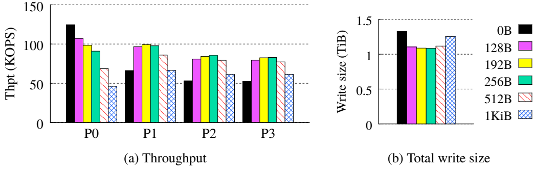
Figure 13: Experiment 8: Threshold selection of selective KV separation in HashKV under update-intensive workloads.
