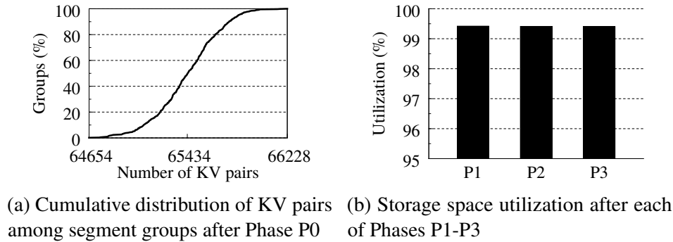
Figure 19: Experiment 14: Storage distribution of KV pairs in HashKV.
