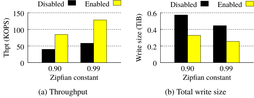
Figure 11: Experiment 6: Hotness awareness.
