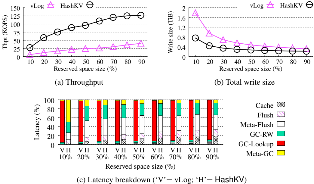
Figure 7: Experiment 2: Impact of reserved space size.
