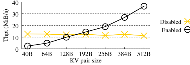
Figure 5: Update throughput versus the KV pair size with and without KV separation.
