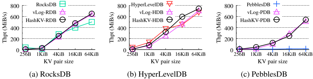
Figure 18: Experiment 13: Impact of KV separation on different KV stores under range scan workloads.
