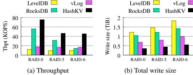
Figure 8: Experiment 3: Different RAID configurations.
