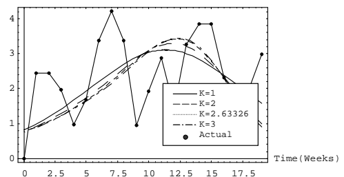
Figure 1: Observed/estimated testing-effort vs. time for the first data set.
