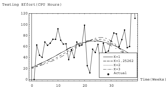
Figure 3: Observed/estimated testing-effort
