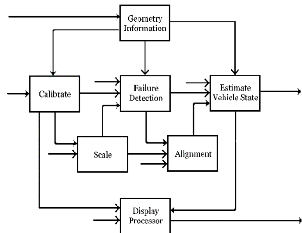
Figure 1 RSDIMU System Data Flow Diagram
