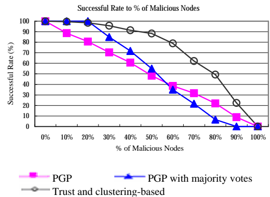
Figure 5. Comparison on successful rates
