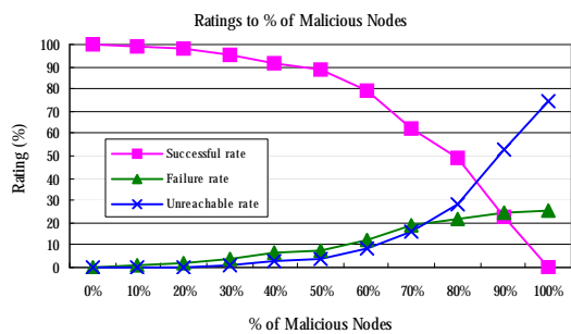
Figure 4. Ratings to percentage of malicious nodes
