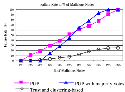
Figure 6. Comparison on failure rates
