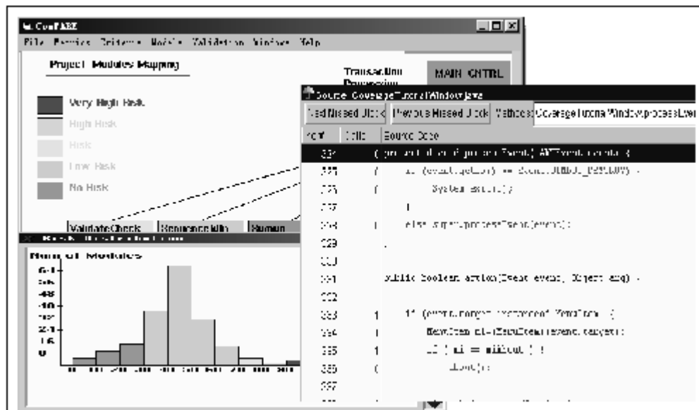
Figure 4. GUI of ComPARE for prediction display, risky source code and result statistics
