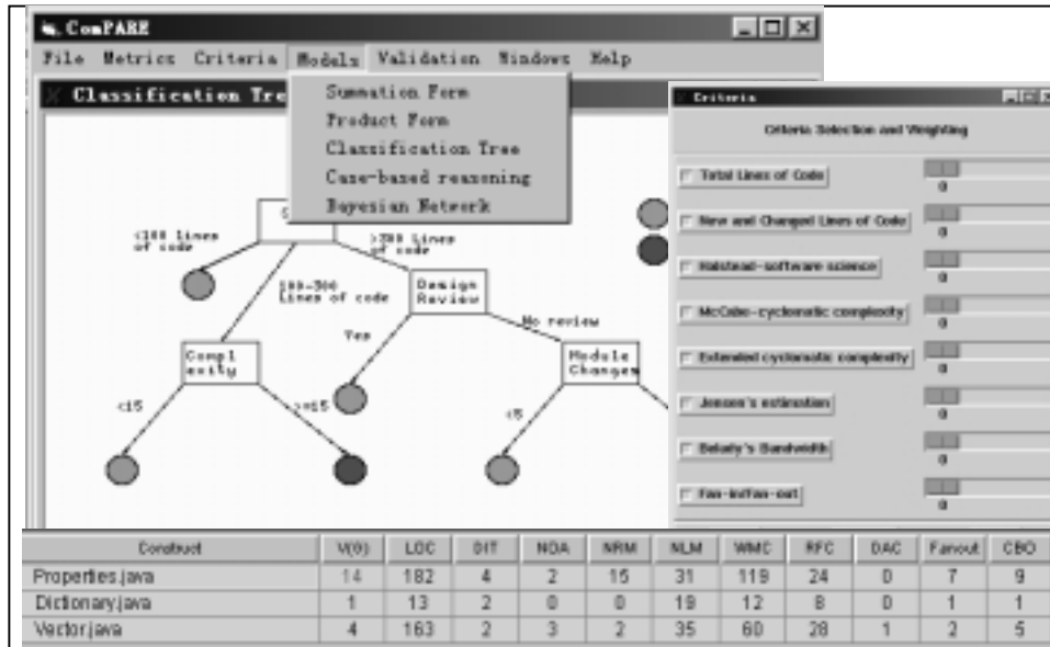
Figure 3. GUI of ComPARE for metrics, criteria and tree model
