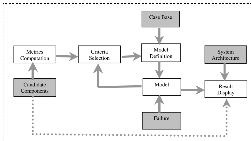
Figure 1. Architecture of ComPARE
