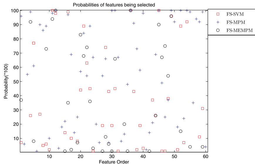
(b) Probabilities of features being selected in sonar
