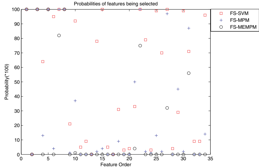
(a) Probabilities of features being selected in iono
