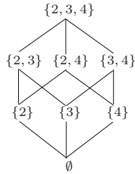
Figure 2: The modified set domain of S .
