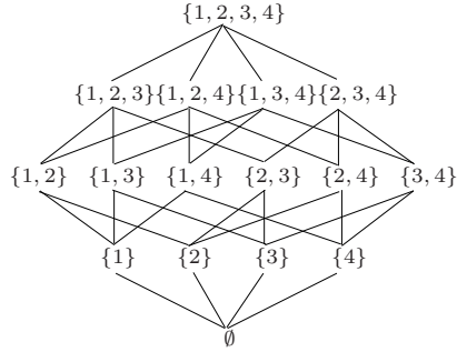
Figure 1: The domain of a set variable S with interval [\emptyset, \{1, 2, 3, 4\}]
