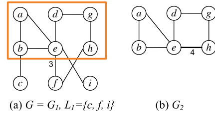
Figure 3: A k -level vertex hierarchy ( k = 2 )
