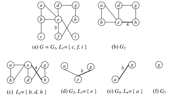
Figure 1: A vertex hierarchy
