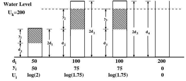
Fig. 2. Example for the Progressive Filling Alg.
