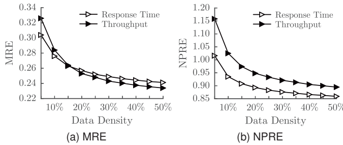
Fig. 12. Effect of Data Density
