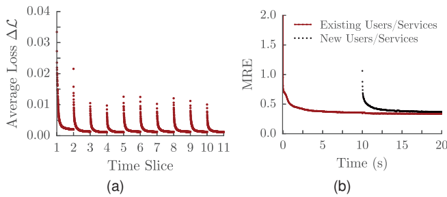
Fig. 14. Robustness Evaluation Result
