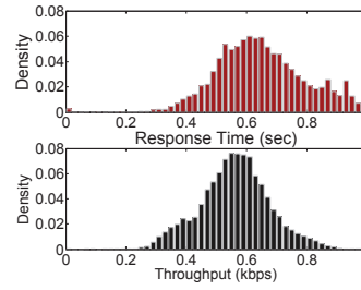
Fig. 8. Transformed Distribution
