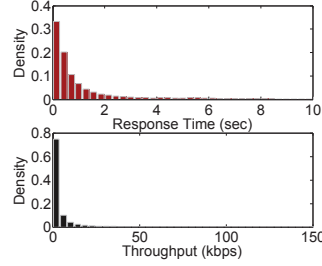
Fig. 7. Data Distribution
