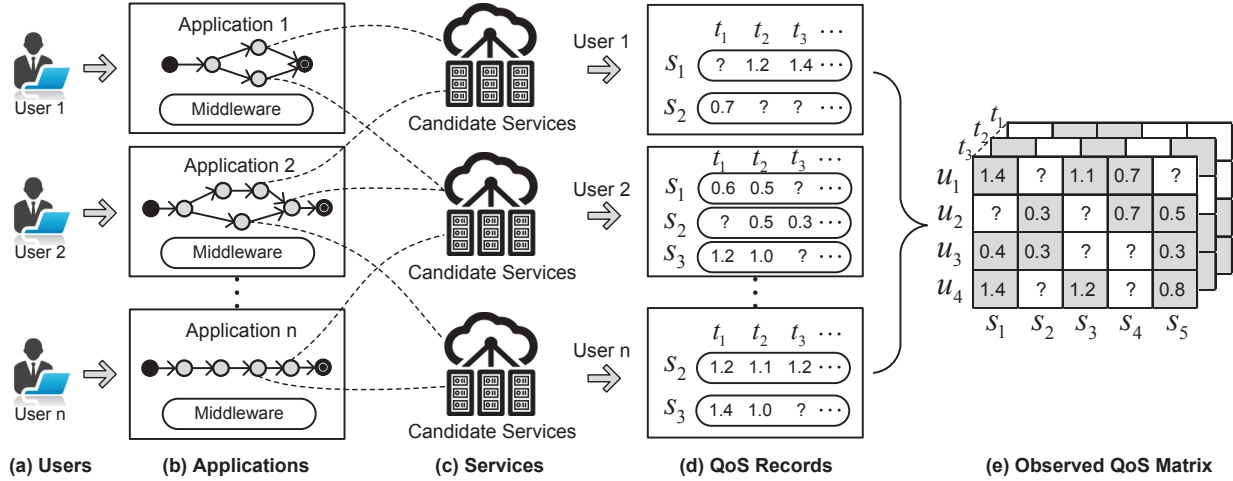
Fig. 4. The Problem Setting of Online QoS Prediction
