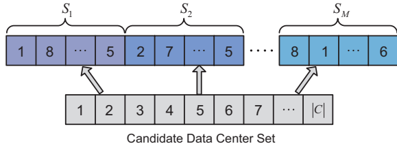
Fig. 2. Genome Encoding of Deployment Strategy
