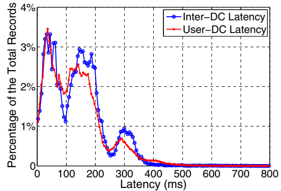
Fig. 3. The Approximate Distributions of Inter-DC Latencies and User-DC Latencies (DC: Data Center)
