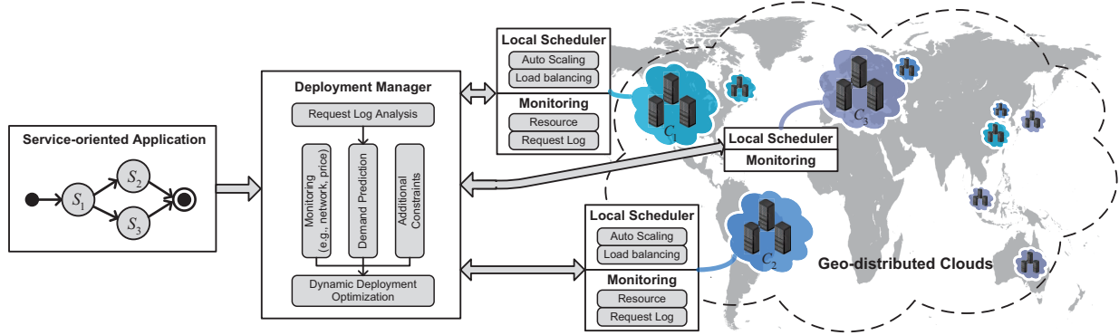
Fig. 1. The Framework of Service-oriented Applications Deployment in Geo-distributed Clouds
