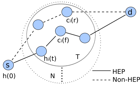
Fig. 1. Illustration of Notations of the Coalitional Game
