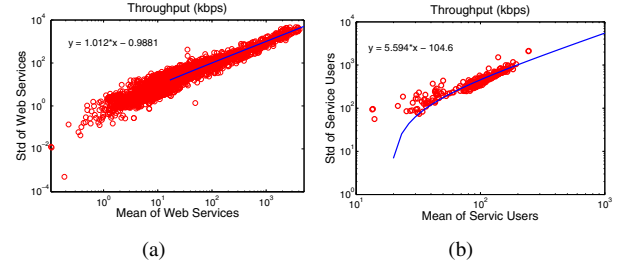
Figure 9. Overall Throughput
