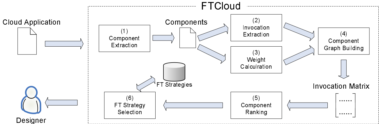
Figure 2. Implementation of FTCloud
