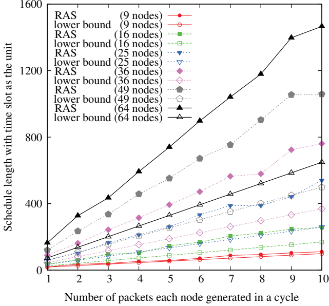
Fig. 3. RAS schedule length vs. lower bound schedule length.
