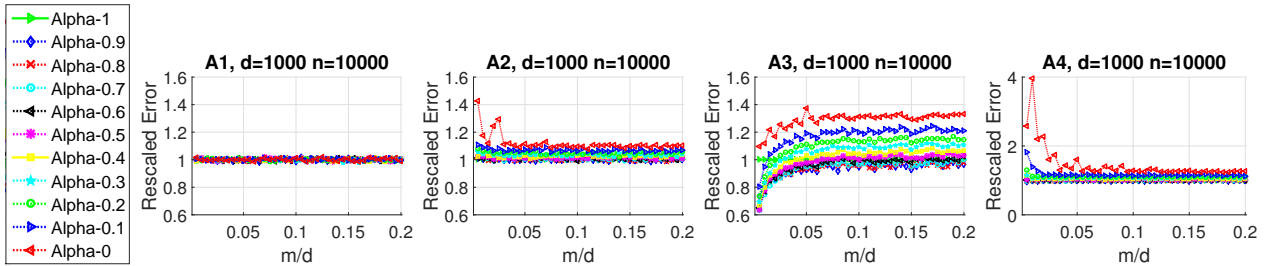
Figure 1. Accuracy comparison by decreasing \alpha from 1 to 0 with a step size of 0.1. The error at each \alpha is normalized by that at \alpha = 1 on y -axis, and m/d varies from 0.005 to 0.2 with a step size of 0.005 on x -axis. Roughly, \alpha = 0.9 is a good choice, and the smaller parameter like \alpha = 0 usually leads to a poorer accuracy and higher variance compared with the other \alpha values.
