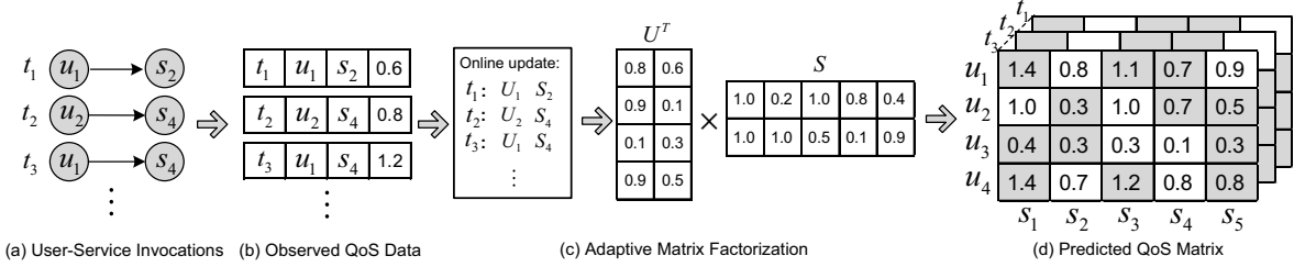
Fig. 5. An Example of QoS Prediction by Adaptive Matrix Factorization
