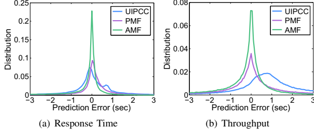
Fig. 10. Distribution of Prediction Errors
