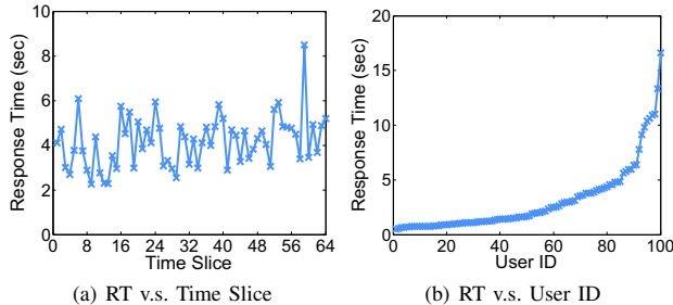
Fig. 2. Real-world Response Time (RT) Observations
