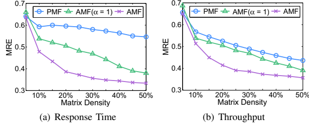
Fig. 11. Impact of Data Transformation
