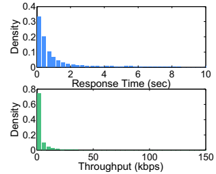
Fig. 7. Data Distribution
