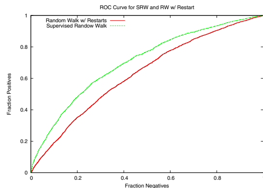
Figure 8: ROC curve of Astro-Ph test data.
