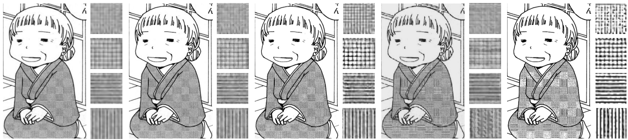
(a) Degraded manga (b) EDSR[14](200%) (c) SRGAN[12](200%) (d) MetaSR[8](127%) (e) Ours(127%)
