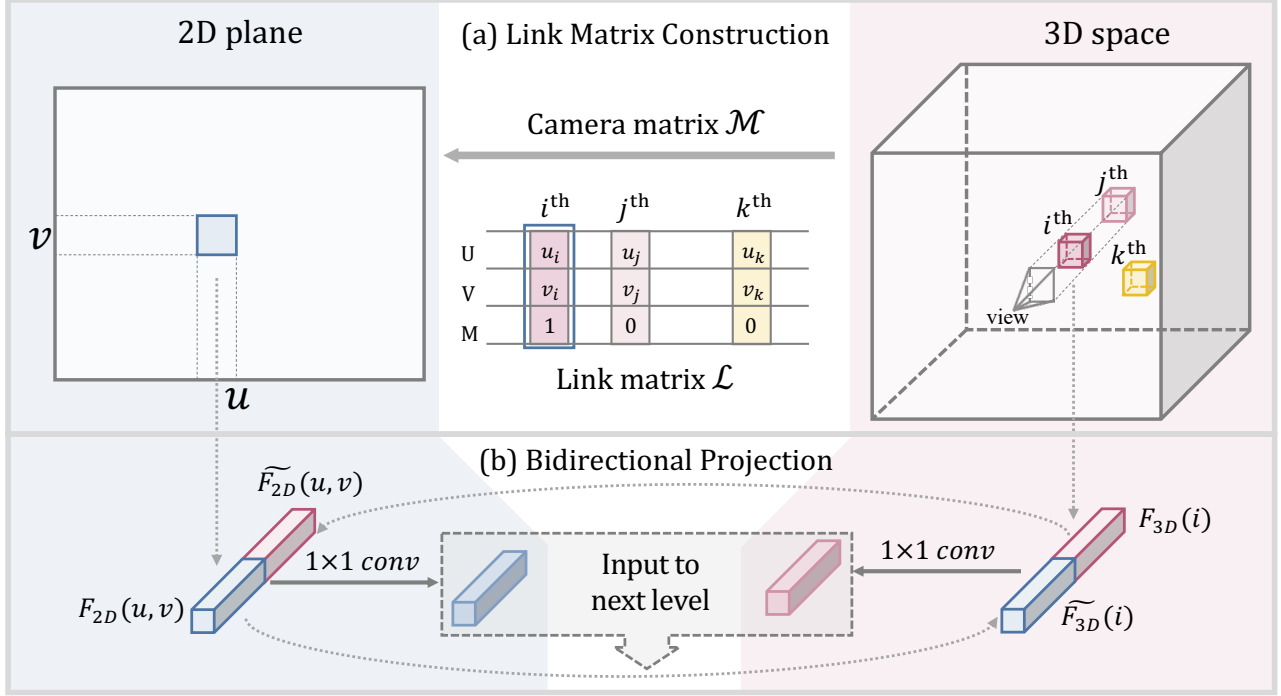
Figure 2. Bidirectional Projection Module (BPM). The link matrix construction procedure between one view and the 3D scene is illustrated in (a), and the bidirectional projection procedure is shown in (b). \mathcal{M} is the camera matrix; the i^{\text{th}} , j^{\text{th}} and k^{\text{th}} voxels are typical examples of three kinds of voxels: voxels that have corresponding pixels under this view, voxels that are occluded by others, and voxels that are out of the view frustum. F_{2D} and F_{3D} are features in 2D and 3D spaces, respectively. \widetilde{F}_{2D} and \widetilde{F}_{3D} are the 2D and 3D bidirectionally projected features from the other domain, respectively.
