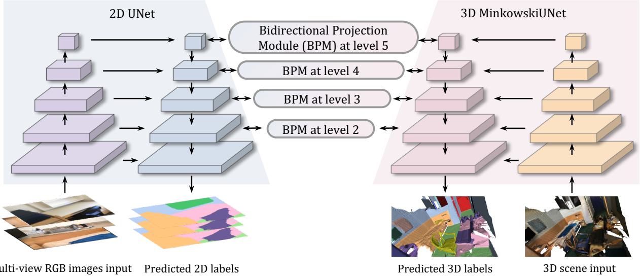
Figure 1. Overview of the Bidirectional Projection Network (BPNet). It consists of two symmetric sub-networks, 2D UNet [46] (in the left-hand side) and 3D MinkowskiUNet [6] (in the right-hand side). Both the 2D and 3D sub-networks are the U-shaped network with the same number of pyramid levels, but they are constructed based on conventional 2D convolution and 3D sparse convolution [12], respectively. At multiple pyramid levels in the decoder stage, the features interact bidirectionally between 2D and 3D sub-networks via the proposed Bidirectional Projection Module (BPM). Both 2D and 3D semantic labels will be predicted simultaneously by our BPNet.
