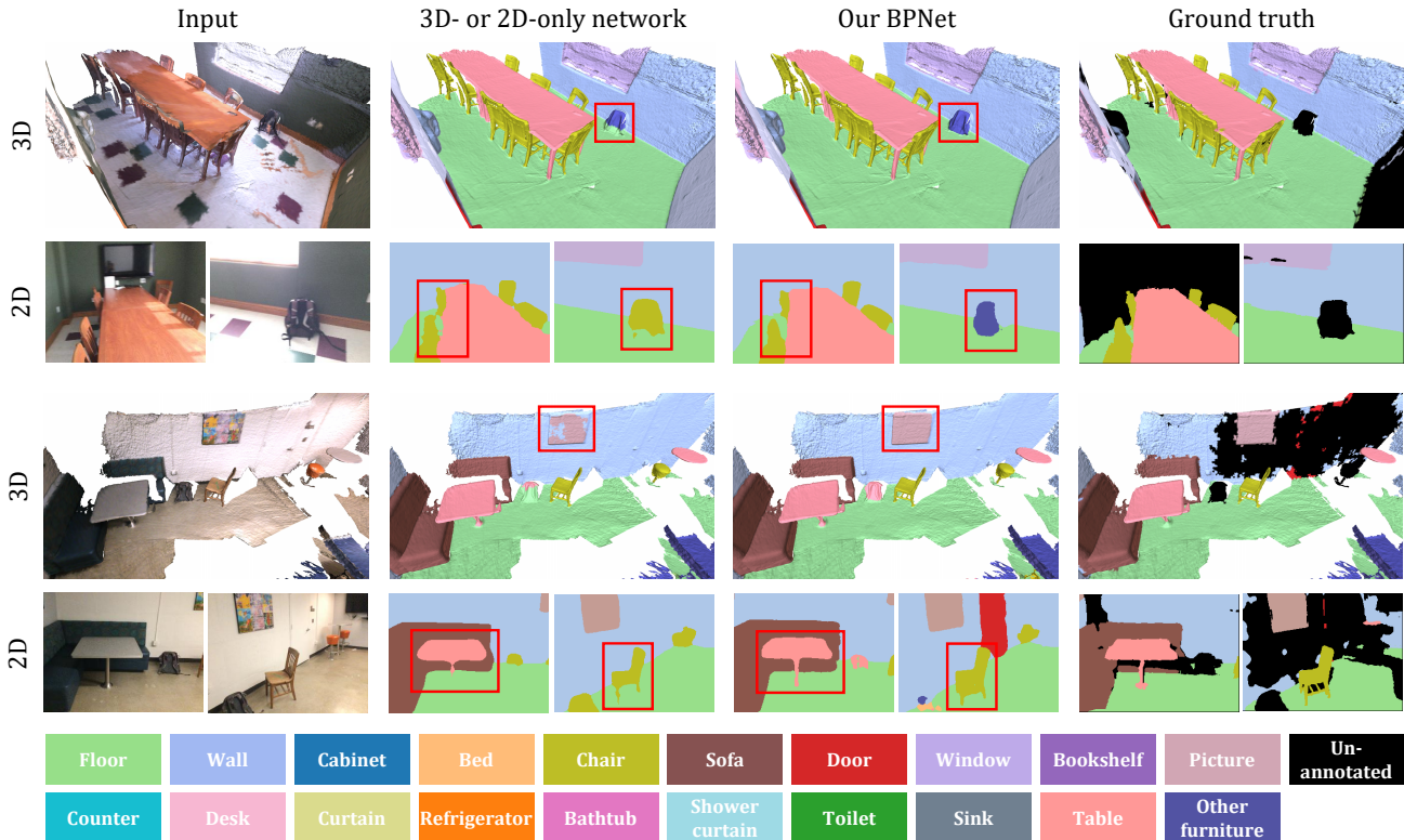
Figure 3. Qualitative 3D and 2D result examples of the 3D-only network, MinkowskiNet [6], 2D-only network, UNet34, our BPNet, and the ground truths. Different semantics are labeled as corresponding colors as shown in the bottom color palette. We highlight the differences between the results of BPNet and others by red boxes.
