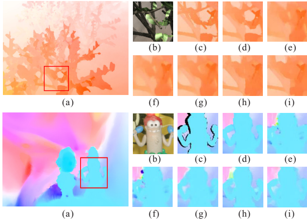
Fig. 13. Visual comparison of the small-displacement optical flow results on two examples. (a) Our flow results. Close-ups of (b) the input image, (c) ground truth flow, (d) our estimate, and of results of (e) Brox et al. [10], (f) LDOF [11], (g) Zimmer et al. [45], (h) Werlberger et al. [38], and (i) of Sun et al. [33], are shown.
