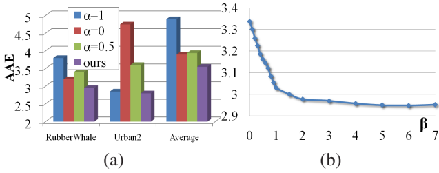
Fig. 8. Flow estimation error comparison. (a) Estimation errors w.r.t. \alpha . \alpha = 1 and \alpha = 0 indicate respectively that only the color or gradient constancy constraint is used. \alpha = 0.5 refers to weighted addition of the two constraints. (b) Estimation errors w.r.t. \beta on the “RubberWhale” example.
