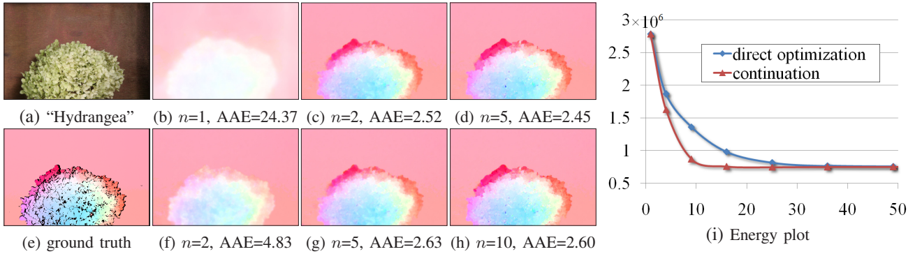
Fig. 6. Continuation scheme. (b)-(d) show our results obtained using the algorithm in Table 2 with the continuation scheme. n is set to 1, 2, and 5 respectively. The error is already very small when n = 2 . (f)-(h) show results with fixed \eta = 0.1 and \theta = 0.01 in all iterations. AAE stands for “average angular error” [3]. (i) Energy decreasing w.r.t. the number of iterations with and without continuation.
